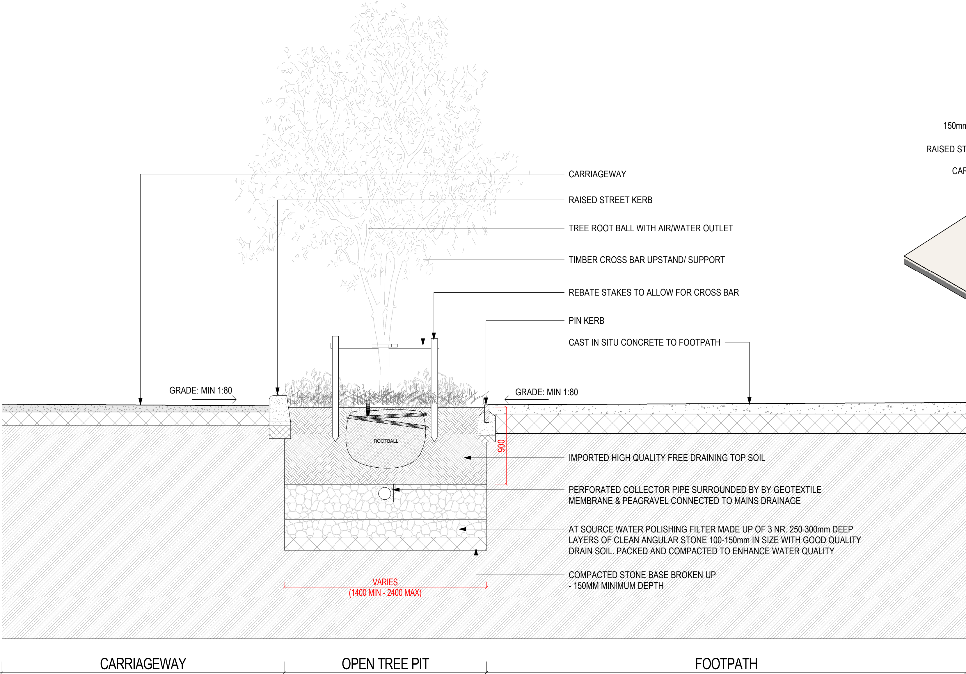
1 TYPICAL TREE PIT 1:25 @A1
