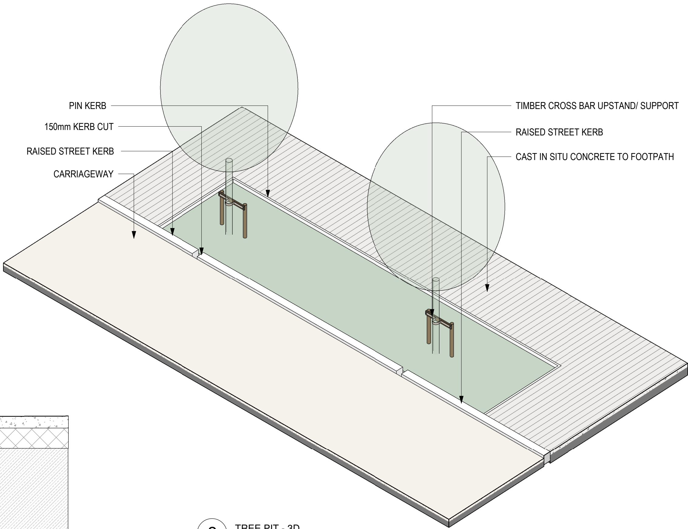
2 TREE PIT - 3D @A1
