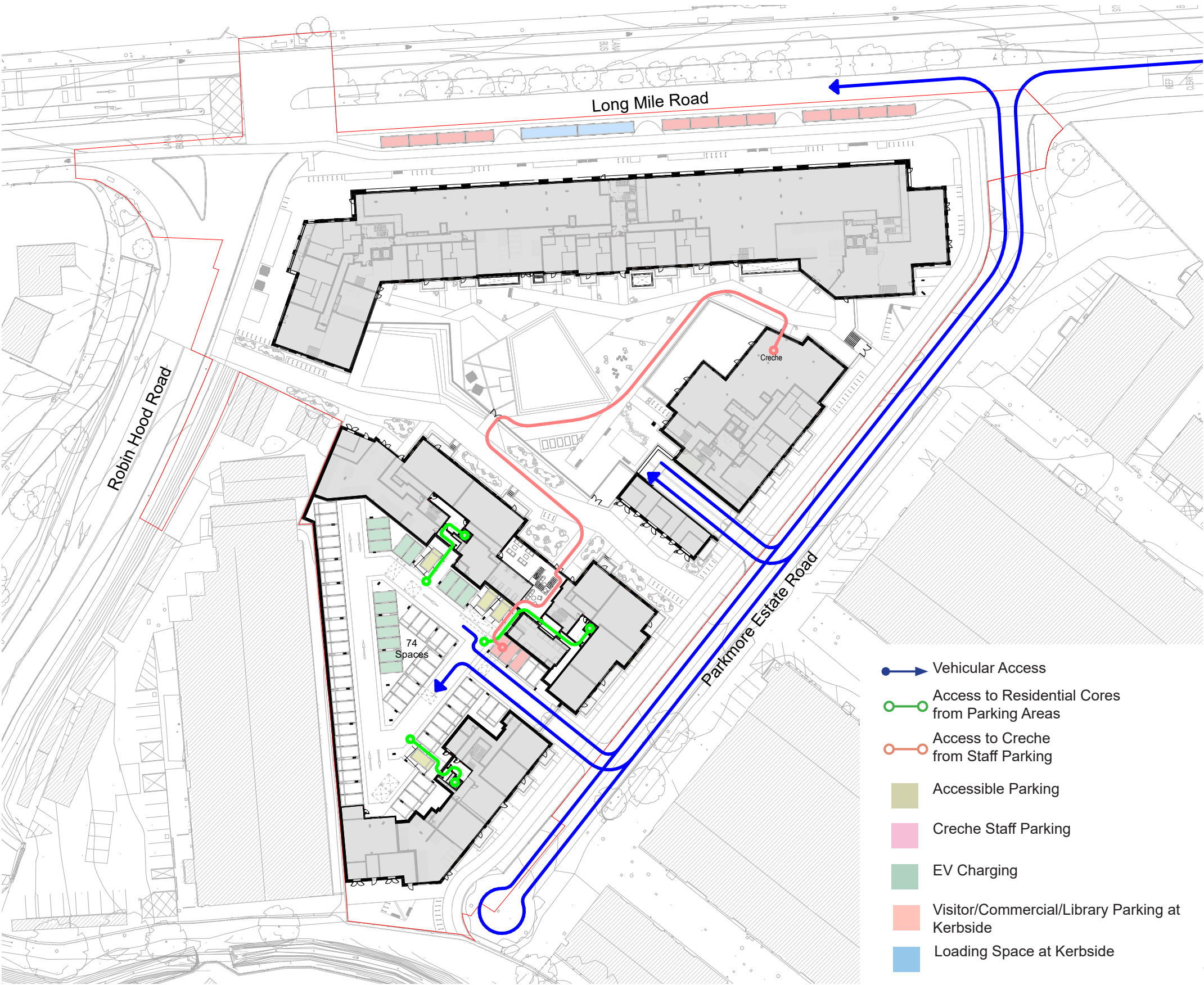
Figure 30 - Ground Floor Plan showing Car Parking areas and Building Access Points.
