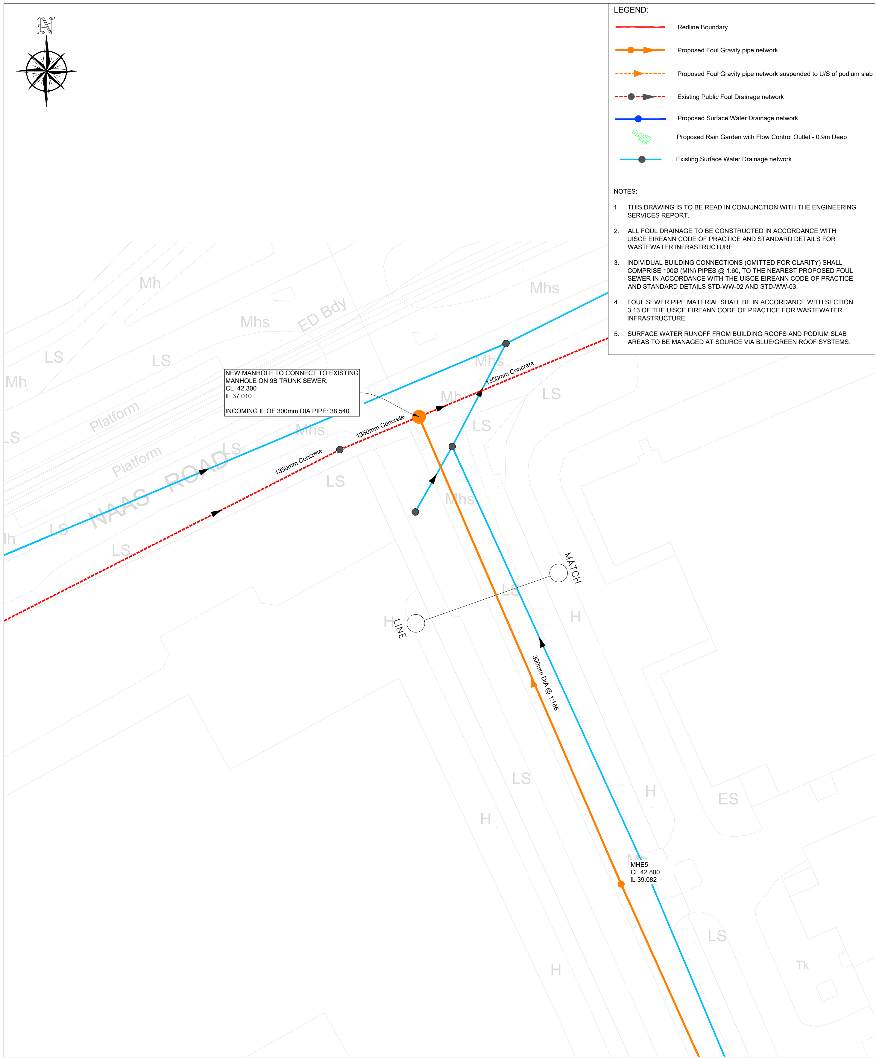
PLAN LAYOUT SCALE 1:400@A1
