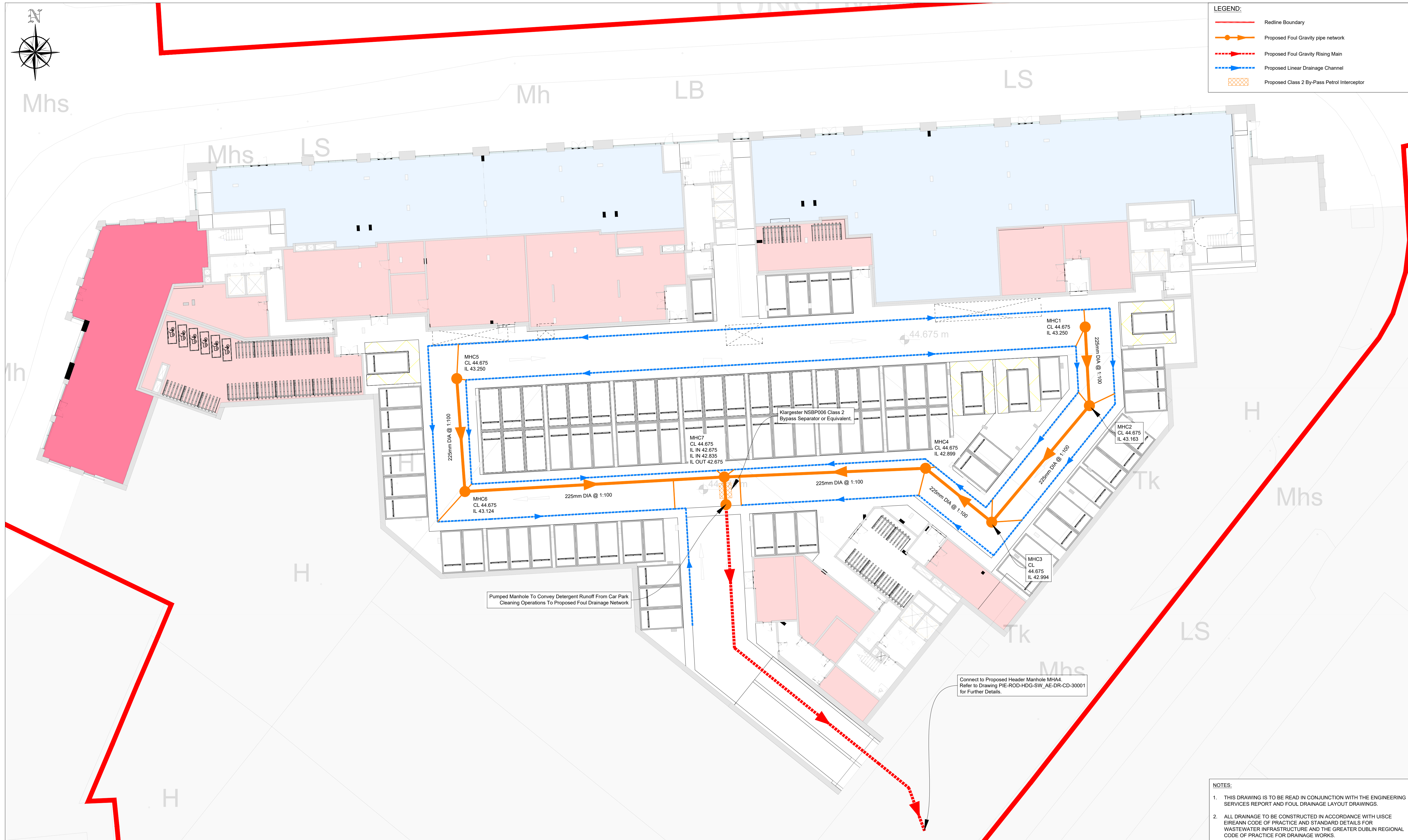
PLAN LAYOUT SCALE 1:200@A1
